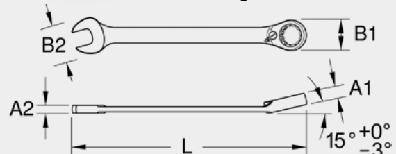
BT013806... 832 Ratchet ring spanner, reversing
